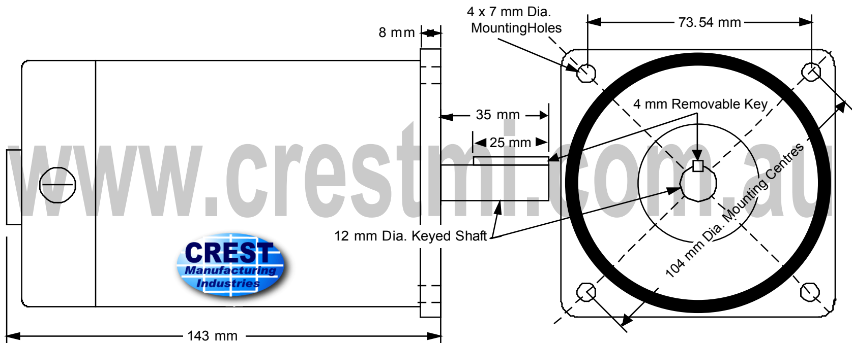
Z5D120 Watt 12 & 24 Volt Precision DC PM Motor Type A1 - Keyed Shaft
